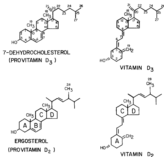
Fig. 1. Structure of vitamin \text{D}_3 and \text{D}_2 and their respective precursors, 7-dehydrocholesterol, and ergosterol. The only structural difference between vitamin \text{D}_2 and \text{D}_3 is in their side chains; the side chain for vitamin \text{D}_2 contains a double bond between C-22 and C-23 and a C-24 methyl group. (Reproduced with permission) [MacLaughlin and Holick, 1983].
